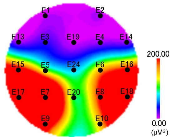
FIGURE 5 Relationship between the topogram and electrode arrangement. The bar on the right indicates electrode power with colors. The upper base is 200 \mu\text{V}^2 (red) and the lower base 0 \mu\text{V}^2 (purple). In this example, a range from red to yellow is seen near E5, E6, E7, E8, E9, E10, E15, E16, E17, and E18, indicating specific potential activity
