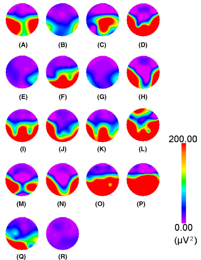
FIGURE 7 Myogenic potential topograms of participants A to R for the voluntary facial expression of happiness: topograms in the range of 30-40 Hz when the upper limit was set at 200 \mu\text{V}^2 . Participants A, C, D, F, H, I, J, K, L, M, N, O, P, and Q, red spread from the bottom of the topogram. Low potential changes are seen in participants B, E, G, and R
