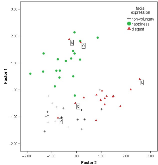
FIGURE 4 Scatter plot of factor scores 1 and 2 for the three facial expressions
