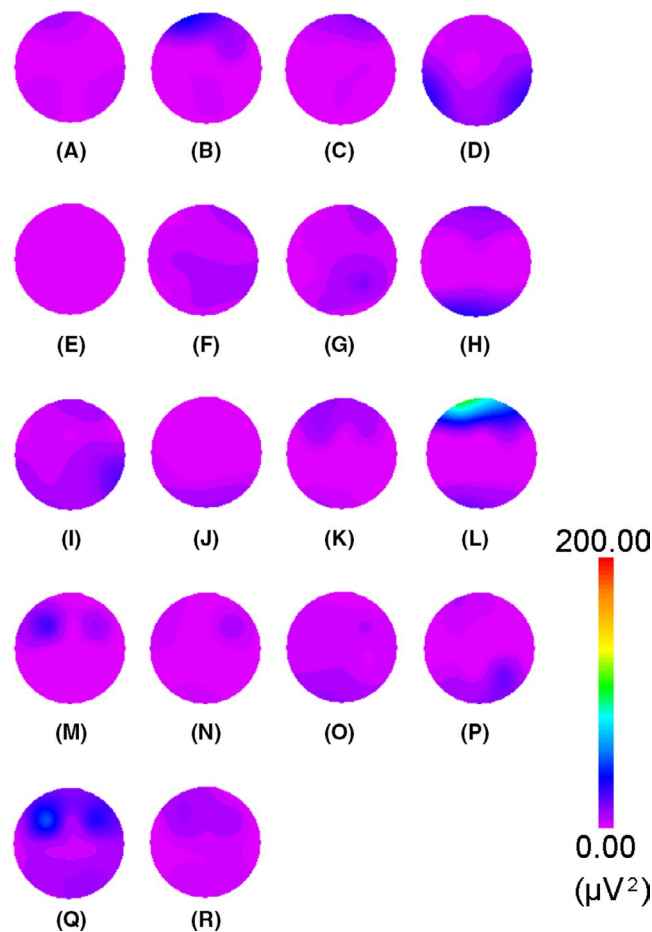
FIGURE 6 Myogenic potential topograms of participants A to R for nonvoluntary facial expression: topograms in the range of 30-40 Hz when the upper limit was set at 200 \mu\text{V}^2 . A range from purple to bluish-purple is seen, indicating no specific changes
