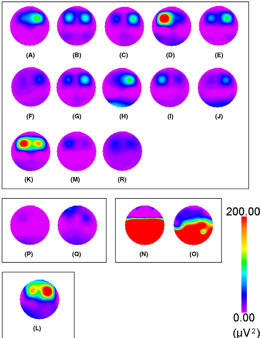
FIGURE 8 Myogenic potential topograms of participants A to R for the voluntary facial expression of disgust: topograms in the range of 30–40 Hz when the upper limit was set at 200 \mu\text{V}^2 . In participants D and K, colors ranging from red to light blue expand centering on E3 and E4. In participants A, B, C, E, F, G, H, I, J, M, and R show changes of colors from light blue to green centering on E3 and E4. In participants N and O, red occupies most of the lower part of the topogram. Four groups are categorized based on cluster analysis with PCA. The same group is enclosed in a square. General types: A, B, C, D, E, F, G, H, I, J, K, M, and R, no change type: P and Q, lower facial type: N and O, strong general types: L
