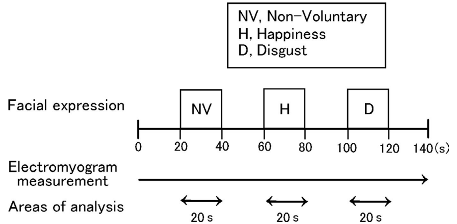
FIGURE 1 Experiment procedure: electromyogram recording. The arrows indicate the analysis scope. Nonvoluntary facial expression, NV ; voluntary facial expression of happiness, H ; voluntary facial expression of disgust, D . Facial expressions were expressed for 20 s, with a 20-s interval between expressions
