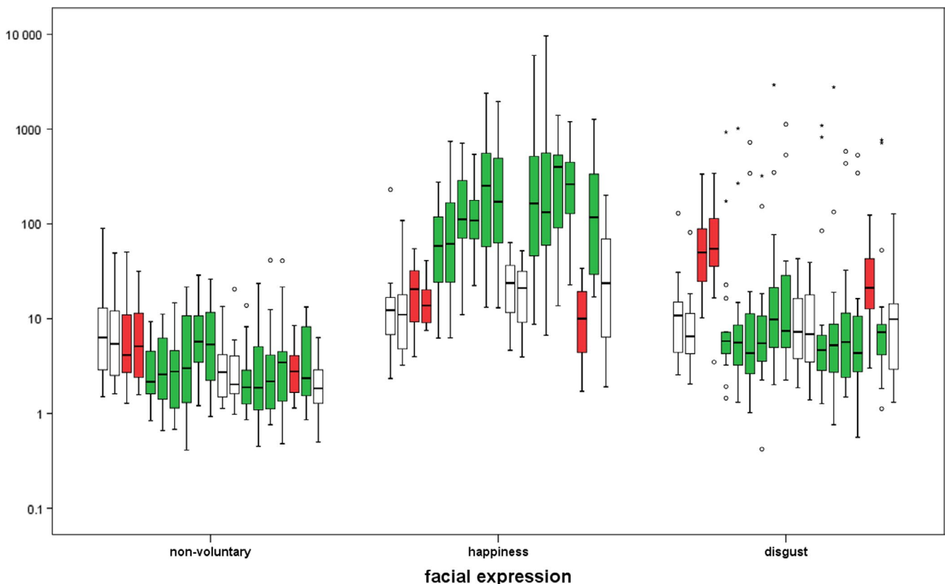
FIGURE 3 Box-and-whisker plot of myogenic potentials in each electrode by facial expression. Changes in myogenic potential are shown in order from the left: E1-E10, E13-E20, and E24. Green: E5-10, E15-18, E20; red: E03, E04, E19; white: the others
