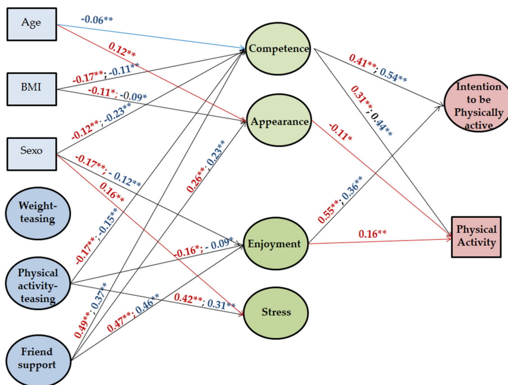
Figure 2. The multi-group final model where standardized parameters of the paths between countries can be compared. Covariances, correlations, and nonsignificant paths are omitted for presentation clarity. Chilean results are in red, Spanish results are in blue. ** p < 0.01 , * p < 0.05 .
