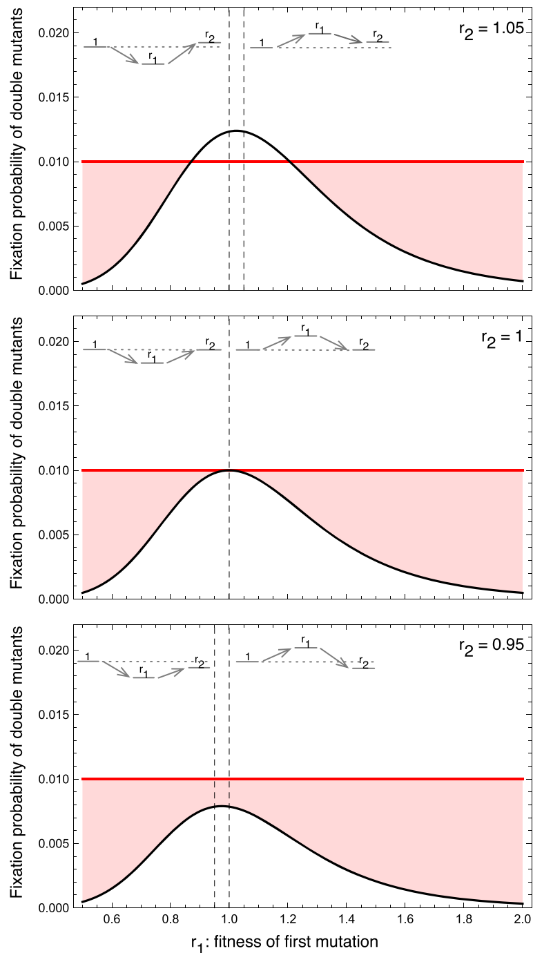
Fig. 3 Fixation probability of two consecutive mutations on the directed line, a suppressor of selection ( red ), and the well-mixed population ( black ) of size N = 10 . This fixation probability is plotted against the fitness of the first mutation. From top to bottom we show an advantageous second mutation ( r_2 = 1.05 ), a neutral ( r_2 = 1 ) and a disadvantageous ( r_2 = 0.95 ) second mutation. The shaded regions show the fitness values for which the fixation probability of the double mutations is higher on the directed line than in the well-mixed population
