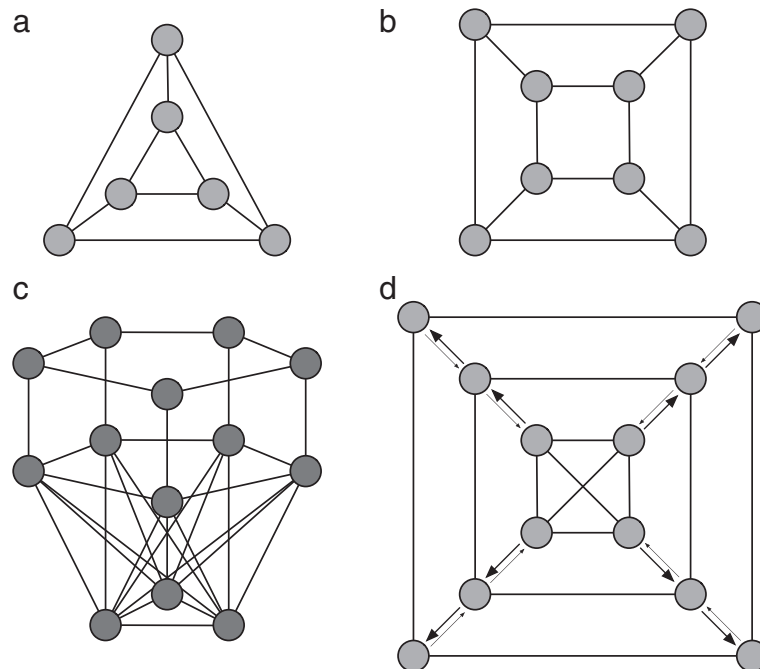
Fig. 2 Different graph structures that can model colonic crypts. a, b Two examples of suppressors of evolution for death-Birth updating. For Birth-death updating, these are equivalent to the well-mixed population in terms of the fixation probability. These two graphs consist of two layers of rings, their qualitative features do not change if we increase these structures to two rings of five, six, up to ten nodes. c This bowl-like graph with 13 nodes comprised of a base of 3 interconnected nodes, which are all connected to all nodes of the middle layer of five nodes. From the middle layer, every node has a corresponding node in the upper ring, to which it is connected. The links are undirected and unweighted. This graph is a suppressor of selection for both Birth-death and death-Birth updating. Thus, it reduces the fixation probabilities for advantageous mutations. d This graph has 12 nodes that are positioned in three layers. Here, the edges are directed and weighted. The outgoing edges between layers have a relative weight of 0.9, whereas the corresponding incoming weights are 0.1. This is to account for the outflowing cell-replacement of the colonic crypt. All other edge weights are 1. This graph is a suppressor of selection for Birth-death and death-Birth updating. The outflowing dynamics makes the suppression even stronger than in the same graph with unweighted edges
