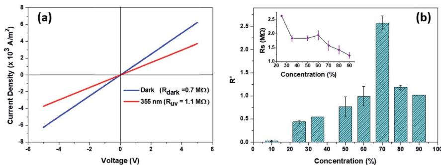
Fig. 2 (a) IV characteristics under dark conditions and UV illumination of the device with ZNP-50 wt%. (b) Histogram showing the variation of fractional PR [ R' = (R_{\text{UV}} - R_{\text{dark}})/R_{\text{dark}} ] with the concentration of ZnO nanoparticles. Error bars indicate the variation in measurements across 5 samples. The inset shows the sheet resistance in the dark of the NC with different ZNP concentrations.
