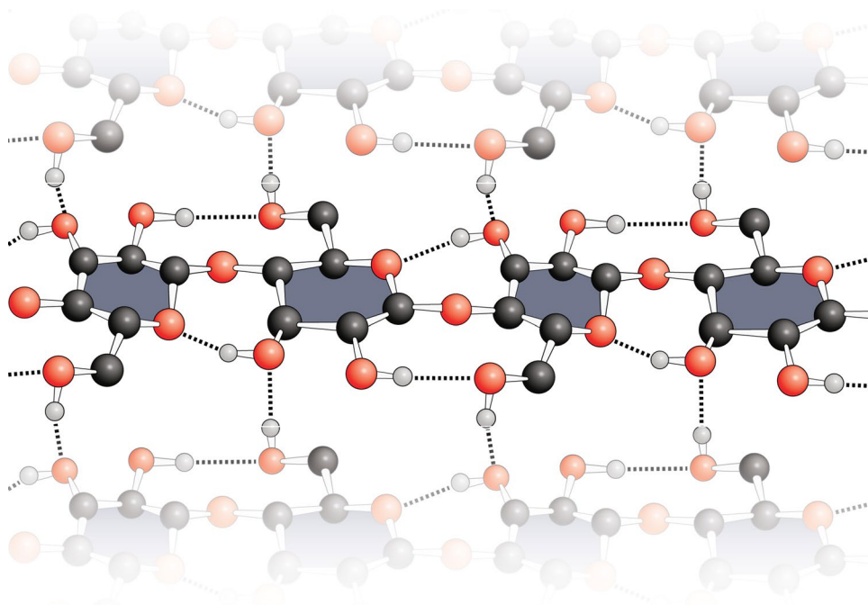
Fig. 5 In cellulose, matched arrays of hydrogen bond donors and acceptors stabilize the folding of (1–4) polymerized glucose into homogeneous fibers. The \beta -anomer but not the \alpha -anomer enables complementary glucose–glucose interactions in the polymer
