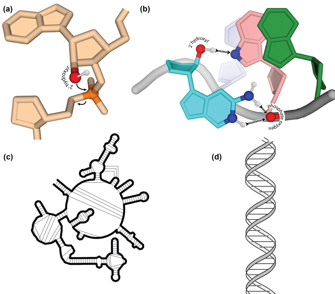
Fig. 6 The impact of the 2' hydroxyl group on polynucleotide reactivity and structure. a Reactivity. RNA holds a gun to its own head. The 2' oxygen is a nucleophile that is poised to attack the adjacent phosphorous atom, cleaving the RNA backbone. b Folding. The 2' hydroxyl group nucleates folding of complex structures by enabling hydrogen bonding between the backbone and bases, as demonstrated in the GNRA tetraloop. The 2' hydroxyl of a guanine forms a hydro-
