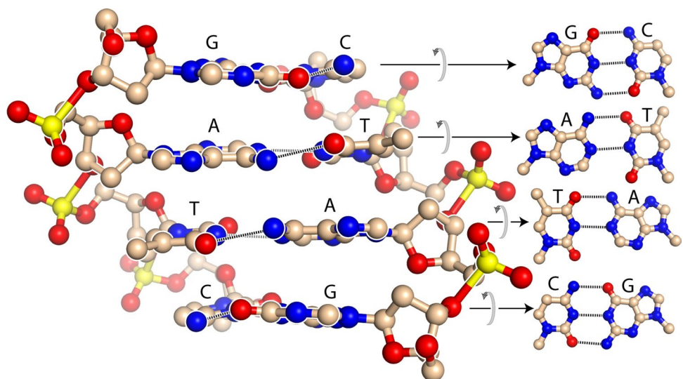
Fig. 4 The DNA duplex with sequence GATC in each strand is self-complementary, containing geometrically matched arrays of hydrogen bond donors and acceptors that link the two strands. On the left, the normals of the base pairs are within the plane of the page. On the right the normals of the base pairs are orthogonal to the page. Hydrogen bonds are indicated by dashed lines
