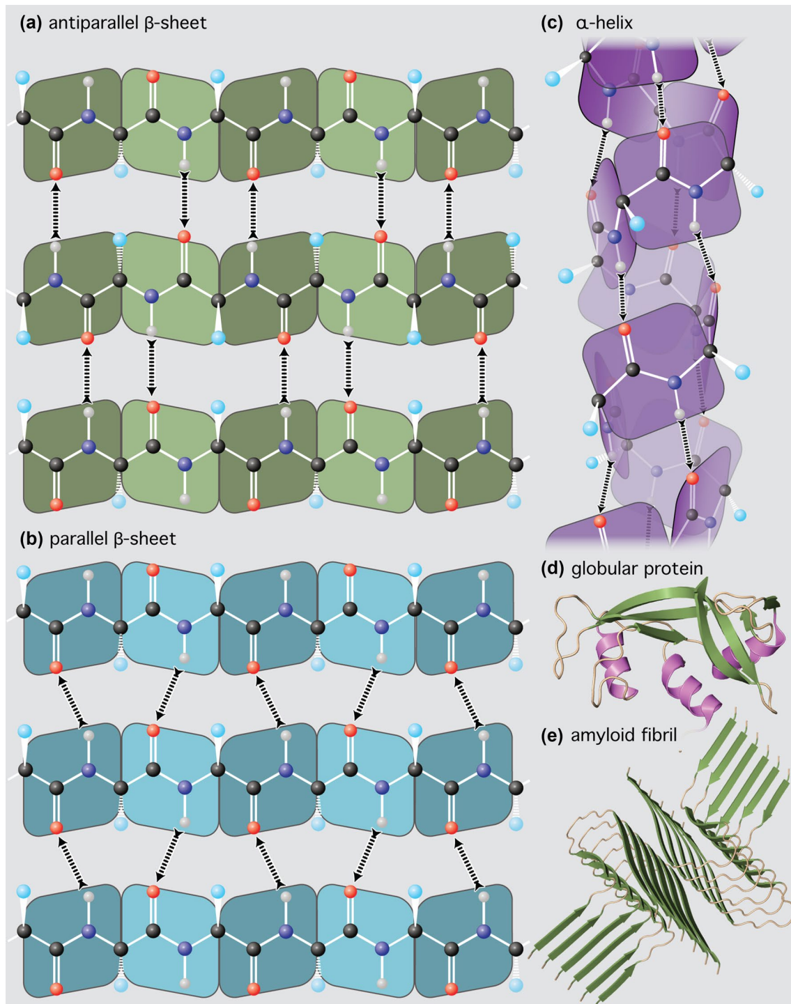
Fig. 3 The self-complementarity of peptide linkages is the dominant molecular interaction in protein secondary structures and in folded protein. a Antiparallel \beta -sheet. b Parallel \beta -sheet. c \alpha -Helix. d A globular protein showing \alpha -helices (violet) and \beta -sheets (green). e
