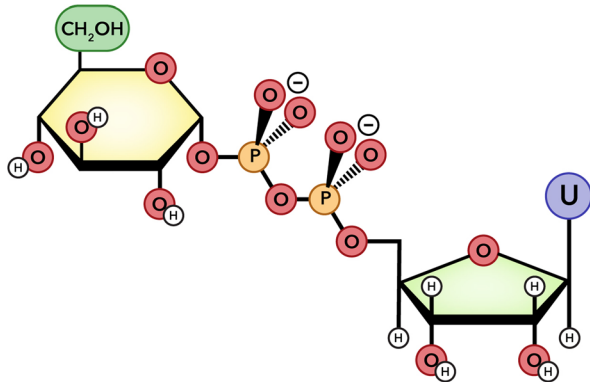
Fig. 2 Intermediates in the biosynthesis of a protein and b polyglucose
