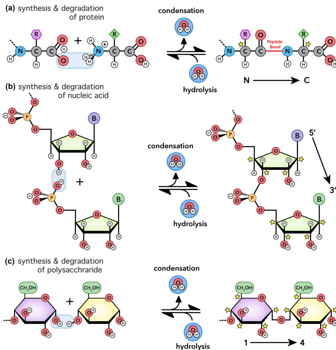
Fig. 1 Net reactions for biopolymer formation by condensation dehydration and biopolymer degradation by hydrolysis. a Protein. b RNA. c Polysaccharide. All biopolymers are chiral and directional with distinctive ends. Chiral centers (stars, shown in polymers only) and
