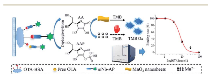
Scheme 1 Schematic illustration of the enzyme cascade-amplified immunoassay based on Nb-AP fusion and \text{MnO}_2 nanosheets for colorimetric detection of OTA in coffee.
