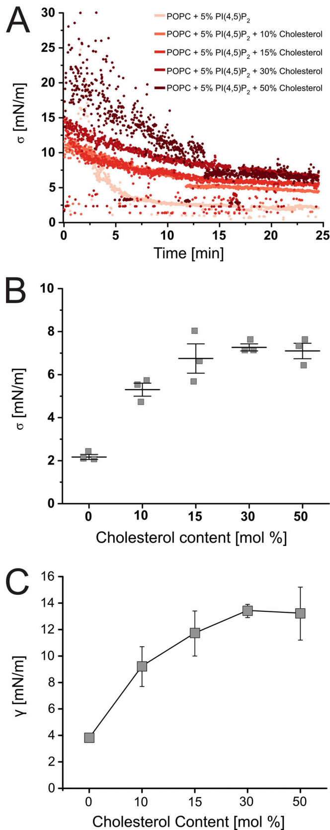
Figure 4. Cholesterol increases membrane tension in PI(4,5)P 2 -containing membranes. (A) Interfacial tensions ( \sigma ) trends measured by pendant drop experiments as a function of time for POPC + 5% PI(4,5)P 2 , varying the cholesterol content (0, 10, 15, 30, 50 mol%). A buffer drop (HEPES
