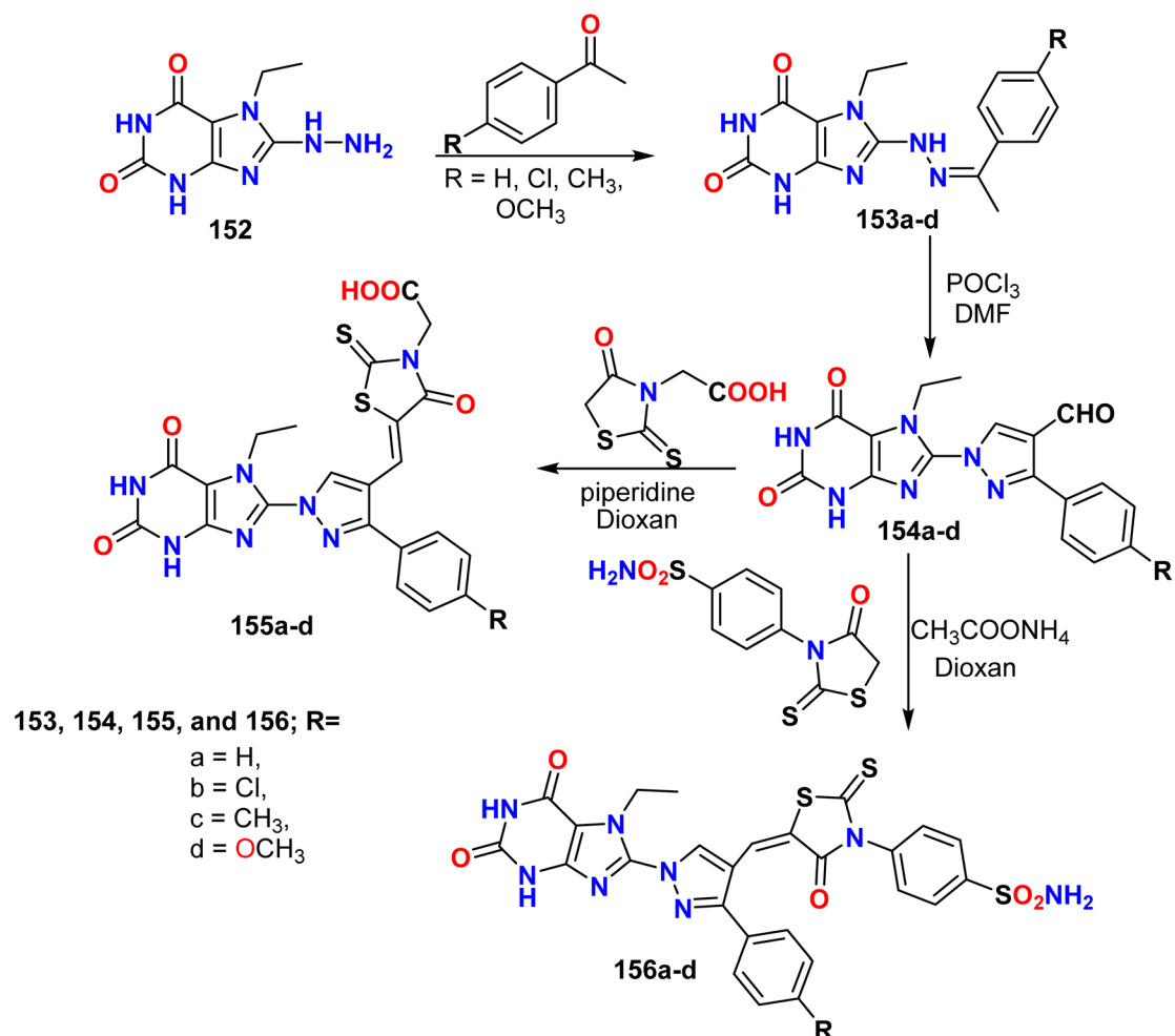
Scheme 41 Synthesis of new Schiff bases based on purine derivatives.
