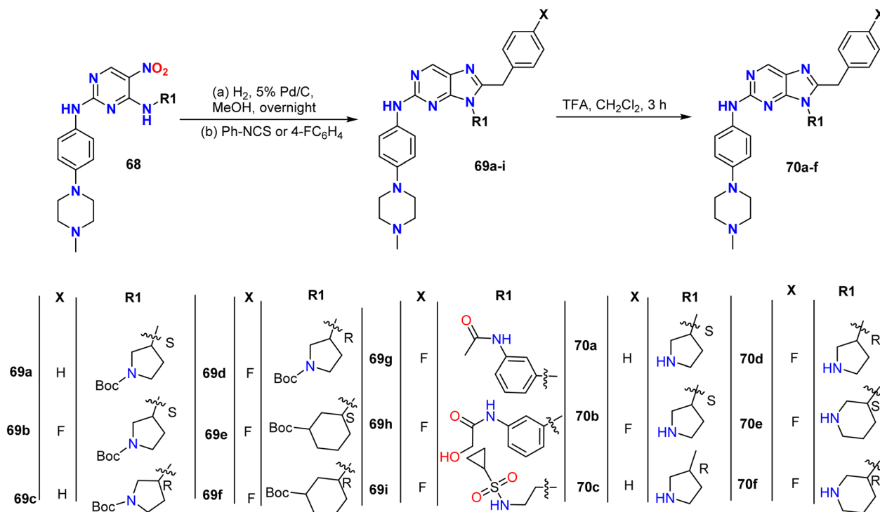
Scheme 17 Synthesis of 9-heterocyclyl substituted 9H-purine derivatives 69 and 70.
