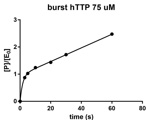
Figure 4. The burst kinetic profile of the incorporation of hTTP at a concentration of 75 μM into the growing duplex P2T3 (100 nM) using T6G12.1521L at a concentration of 14.9 nM as determined via the titration of the enzyme active site. Graphpad Prism v6 was used for data fitting as described in the Materials and Methods section ( R^2 value of 0.997).
