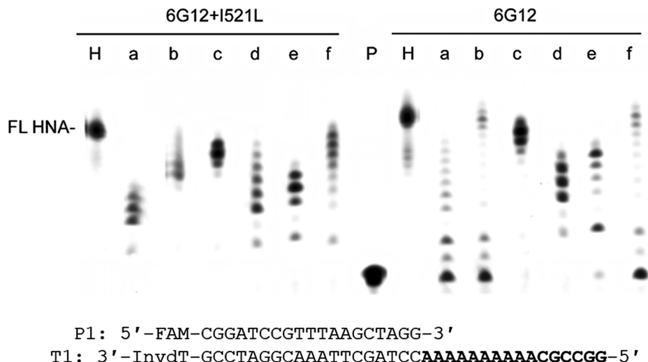
Figure 2. The incorporation of hTTP (H) and the 5-substituted hUTPs 1a-f (lanes a–f) opposite a poly-dA template overhang in a DNA duplex using the evolved HNA polymerases T6G12.I521L and T6G12. The modified nucleotides (hTTP and 1a-f ) are used at a concentration of 125 μM. After optimization of the reaction conditions, the enzymes are used at a final concentration of 51 nM for T6G12.I521L and 82 nM T6G12. The reactions with the enzyme T6G12 contain 0.5 mM freshly prepared MnCl 2 . All reactions are carried out in 1× Thermopol buffer (NEB) supplemented with 1.5 mM MgSO 4 . The reactions are incubated at 50°C overnight. The positions where a 5-substituted hUTP has to be incorporated opposite the template oligonucleotide, are underlined in the sequence below the gel image. The lanes indicated with ‘P’ show the primer control (no enzyme and no nucleotides added). The position for the full-length material of HNA (signifying the incorporation of ten hT nucleotides) is indicated by ‘FL HNA’ on the side of the gel image.
