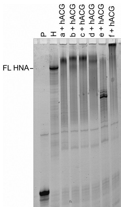
Figure 3. The incorporation of the 5-substituted hUTPs together with hATP, hCTP and hGTP into the PIT2 duplex overhang using T6G12.1521L after cycling for 1 min at 94°C, followed by 5 min at 50°C and 2 h 65°C, for 16 h in total, in Thermopool buffer 1× containing an additional 2 mM MgSO 4 . 'P' indicates the primer control. Lane H shows the hNTP control. Lanes a + hACG to f + hACG show the incorporation of the hA, hC and hG building blocks together with 1a–f respectively.
