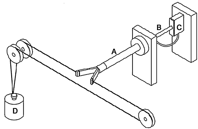
Fig. 7 Schematic drawing of the setup. Shaft A was placed in a clamp and attached to the table. The rod B was attached to the force sensor C. Mass D pulled on the wires that were attached to the tips of the forceps and guided via three pulleys
