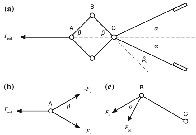
Fig. 3 Kinematics and force propagation of a four-bar mechanism
