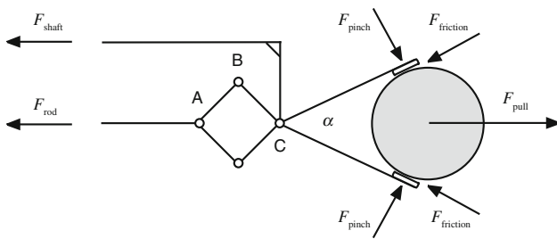
Fig. 2 Schematic representation of the rhombus linkage
