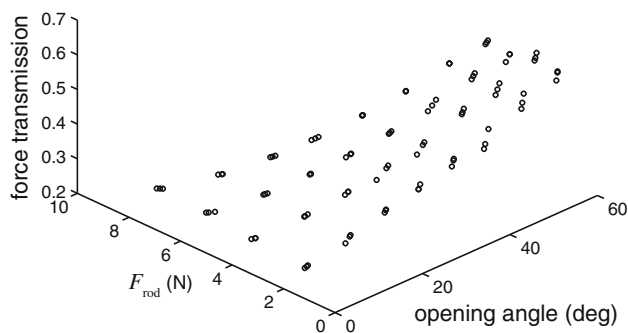
Fig. 9 Force transmission values. Transmission values for different opening angles of the grasper and different forces applied on the rod. Each circle represents a single measurement
