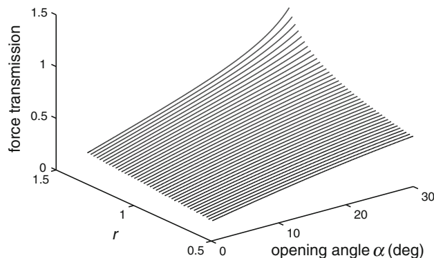
Fig. 5 Force transmission coefficients. Coefficients as a function of opening angle of the grasper for different ratios r between the lengths of the links of the four-bar mechanism
