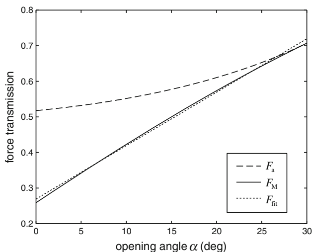
Fig. 4 Force transmission coefficients. The dotted line represents a linear fit to sinusoidal relationship between the force on the rod and the effective force on the link that drives the forceps
