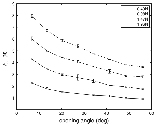
Fig. 8 Forces on the rod. Forces for the different opening angles and forces applied on the forceps. Error bars represent standard deviations around the mean for the three repeated measurements of each combination of opening angle and applied force. Opening angles represent the angle between the two forceps
