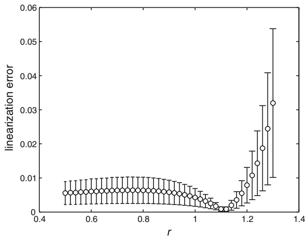
Fig. 6 Linearization errors. Linearization errors for force transmission coefficients for different ratios r between the lengths of the links of the four-bar mechanism. Circles represent values averaged across opening angles. Error bars display standard deviations in the errors
