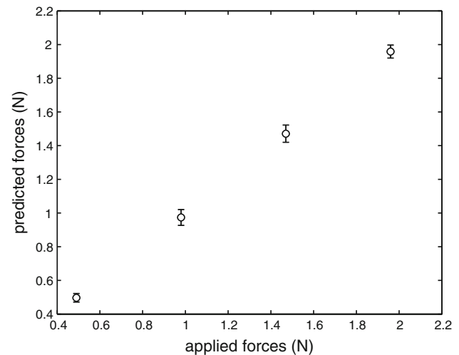
Fig. 10 Predicted forces versus applied forces. The forces on the forceps were estimated from the forces on the rod and the opening angle of the forceps using a two-dimensional linear function. The results are plotted against the actual values used in the experiment. Error bars represent standard deviations in the estimated values across opening angles
