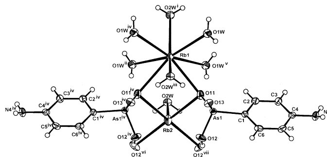
Figure 2 The molecular configuration and atom numbering scheme for the complex unit in the isotopic structure (II). The metal cations (Rb1 and Rb2) and the water molecule ( \text{O}2\text{W} ) also lie on a mirror plane. For symmetry codes, see Table 2. Non-H atoms are shown as displacement ellipsoids at the 40% probability level.
