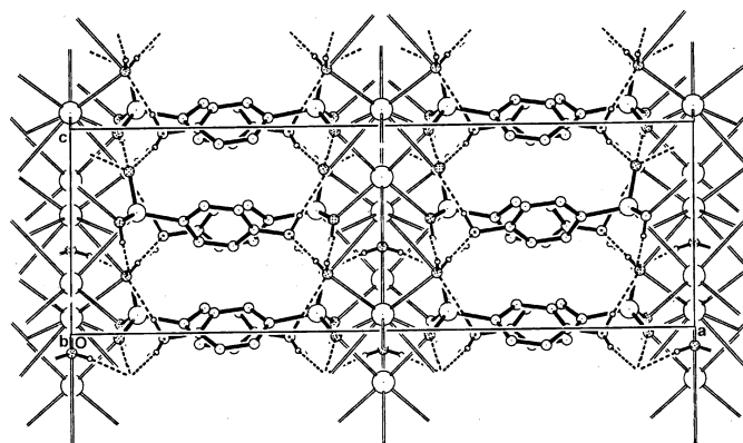
Figure 7 A view of the packing in the unit cell of (II) [or (III)] along [010], showing the associated cation/anion sheets linked peripherally across [100] by hydrogen bonds involving the amine groups.
