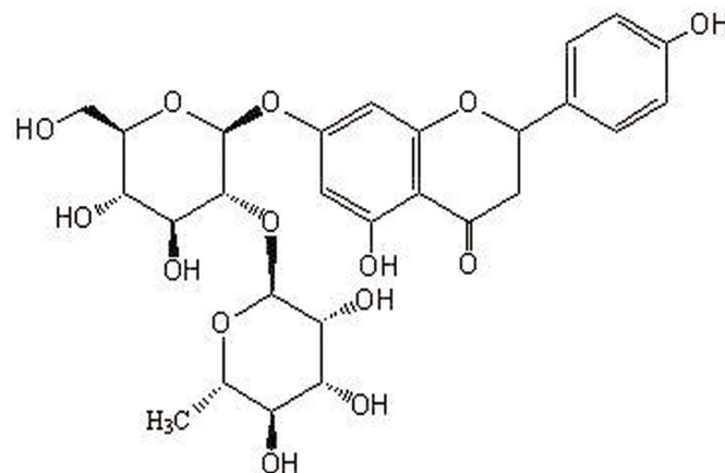
Fig 1. The chemical structure of naringin. The molecular formula of naringin is \text{C}_{27}\text{H}_{32}\text{O}_{14} and the molecular weight is 580.53.
