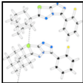
Fig. 2. Partial packing diagram for (I) showing the C—H...S interaction as a dashed line.
