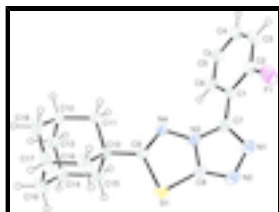
Fig. 1. View of (I) with displacement ellipsoids drawn at the 30% probability level. H-atoms are shown by small spheres of arbitrary radius.
