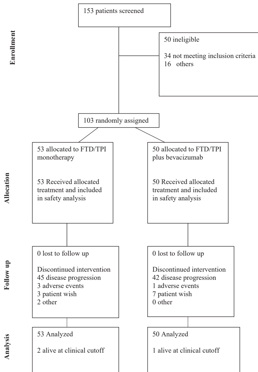
Fig. 1: Consort diagram.
