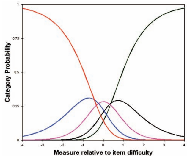
Figure 2. Category probability relative to item difficulty.
