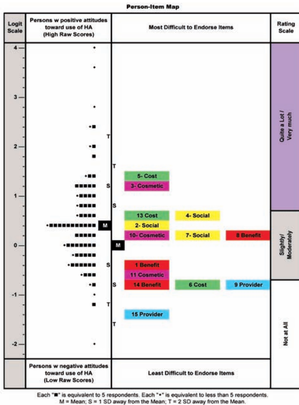
Figure 4. Item map of all subjects and positively/negatively phrased item difficulty.
