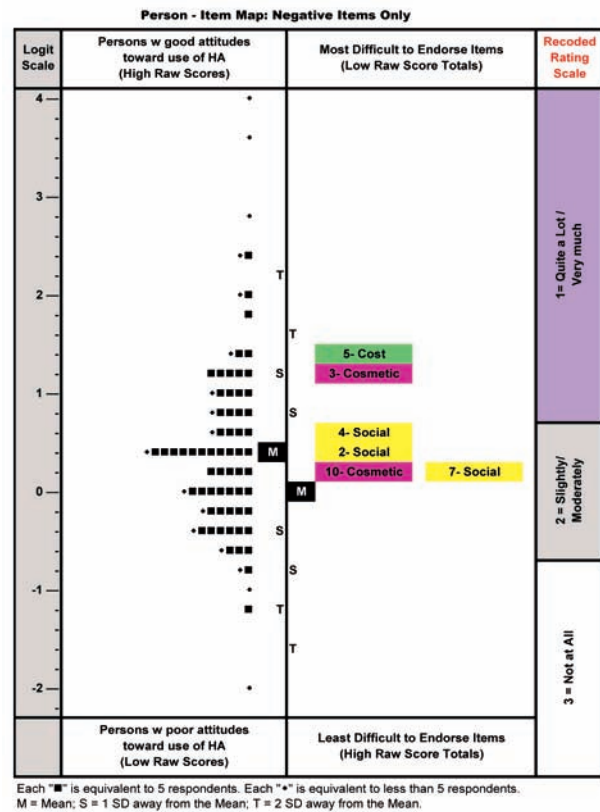
Figure 6. Item map of all subjects and negatively phrased items only.
