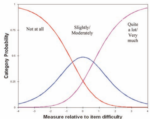
Figure 3. Category probability relative to item difficulty after collapsing two categories.
