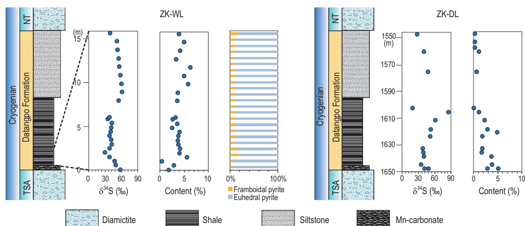
Figure 3. \delta^{34}S_{py} , pyrite content and pyrite morphologies of Cryogenian non-glacial deposits in the Datangpo Formation at ZK-WL and ZK-DL drill cores in South China.
