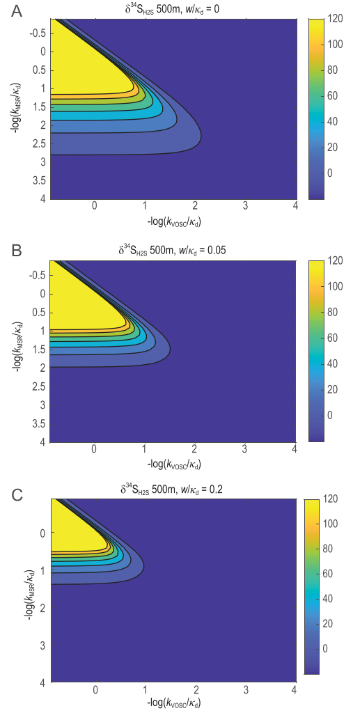
Figure 6. Sensitivity tests to evaluate the influence of microbial sulfate reduction rate constant ( k_{\text{MSR}} ), VOSC generation rate constant ( k_{\text{VOSC}} ) and vertical velocity rate ( w ) on \delta^{34}\text{S}_{\text{H}_2\text{S}} . The X and Y axes represent negative log of k_{\text{VOSC}} and k_{\text{MSR}} , respectively, relative to \kappa_d . The contour lines represent \delta^{34}\text{S}_{\text{H}_2\text{S}} . Modeling results ( w/\kappa_d = 0 \text{ m}^{-1} for (A), w/\kappa_d = 0.05 \text{ m}^{-1} for (B), and w/\kappa_d = 0.2 \text{ m}^{-1} for (C)) show that superheavy pyrite formation requires a high MSR rate, high VOSC formation rate and low vertical mixing rate. Default parameters: initial \delta^{34}\text{S}_{\text{sw}} value of +30‰; \kappa_d = 0.028 \text{ m}^2 \text{ yr}^{-1} .
