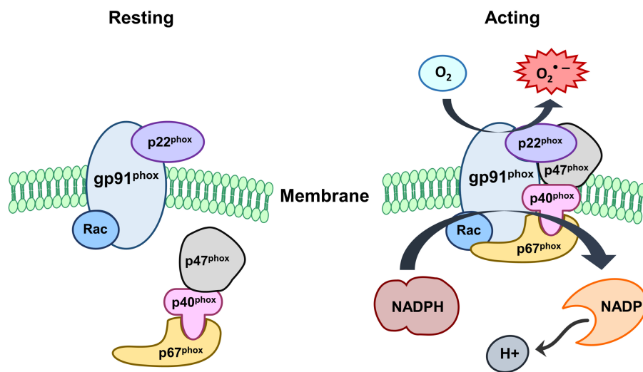
Fig. 1. NADPH oxidase (NOX) activation. NOX comprises cytosolic (p47 phox , p67 phox , p40 phox and Rac) and membrane subunits (gp91 phox and p22 phox ). During activation of NOX, cytosolic subunits comprise a multi-component enzyme and migrate to the plasma membrane to dock with the membrane subunits. This multisubunit enzyme produces a superoxide anion (O 2 •- ).
