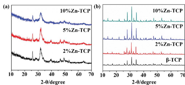
Fig. 3 XRD patterns of (a) the Zn-TCP precursors and (b) the Zn-TCP products.
