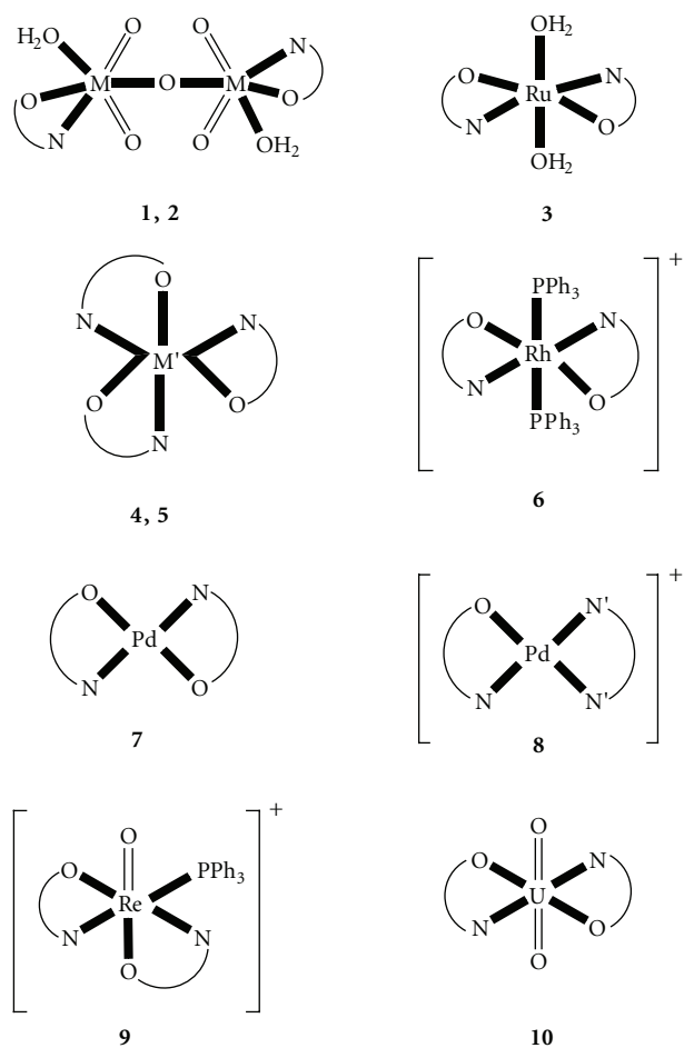
FIGURE 1: Schematic structures proposed for the neutral complexes 1–5, 7, 10 and for the cations of complexes 6, 8, 9. Lattice H 2 O molecules and counterions have been omitted for clarity. However, \widehat{N}\widehat{O} and \widehat{N}'\widehat{N}' represent the ligands L - and phen, respectively. The N and O donor atoms of L - are the amino nitrogen of the position 6 (most probably) and the deprotonated oxygen of the position 5 of the pyrimidine ring; M=Mo, W; M' = Rh, Ir.
