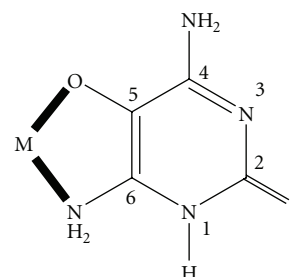
SCHEME 3: The proposed coordination mode of the anionic ligand \text{L}^- in complexes 1–10; \text{M}=\text{metal ion} .
