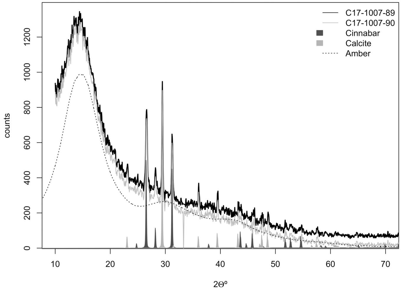
Fig 14. X ray powder diffraction pattern of La Molina samples coatings compared to cinnabar, calcite and amber patterns.
