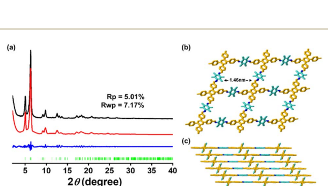
Fig. 3 The experimental and Pawley refined PXRD patterns of TPB-TMPD-COF (a): experimental (black curve), Pawley refined (red curve), difference between experimental and refined patterns (blue curve), and Bragg position from AA stacking with single-pore structure (green curve). Top view and side view of simulated structure for TPB-TMPD-COF (b and c).
