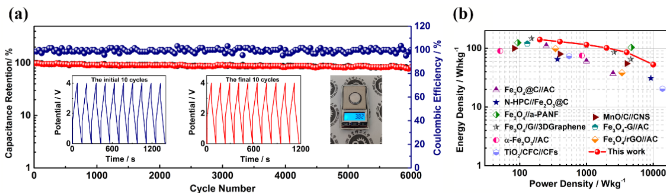
Figure 8. (a) Long-term cycling performance and CE of \text{Fe}_3\text{O}_4@\text{C}//\text{AC} LIC at 2 \text{ A g}^{-1} . Inset: GCD profiles of the initial 10 cycles (blue) and the final 10 cycles (red) and the optical photograph showing the microscale worked by our LIC device; (b) Ragone plots of LIC in our work and other previously reported LICs.
