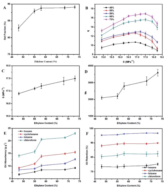
Fig. 5 Effect of ethylene content on the (A) gel fraction, (B) swelling ratio ( q ), (C) solubility parameter ( \delta ), (E) oil-absorption and (F) oil-retention of ESSB; (D) effect of ethylene content on the relative average molecular weight between ESSB cross-linking points.
