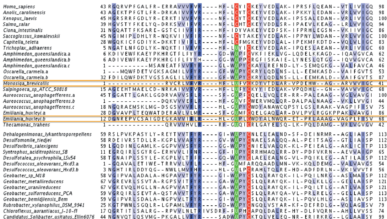
Figure 4. AhpC selenoproteins. Two selenoprotein candidates in our Sebastian predictions were found in M. brevicollis and E. huxleyi , here framed in orange. The figure shows them aligned with other AhpC selenoproteins predicted using Selenoprofiles in eukaryotes (top) and prokaryotes (bottom). Some metazoan cysteine homologues are also shown on the top. The Sec is found in the highlighted redox box UXXC, present also in vertebrates as CXXC. For the full alignment and further details regarding the search for AhpC proteins, see Supplementary Material S6.
