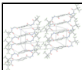
Fig. 2. The crystal packing of the title compound. Hydrogen bonds were shown as dash lines.
