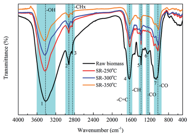
Fig. 4 FTIR spectra of raw biomass and biochars produced from at various HTL temperatures. (1) 3440 \text{cm}^{-1} ; (2) 2923 \text{cm}^{-1} ; (3) 2852 \text{cm}^{-1} ; (4) 1626 \text{cm}^{-1} ; (5) 1384 \text{cm}^{-1} ; (6) 1243 \text{cm}^{-1} ; (7) 1062 \text{cm}^{-1} .
