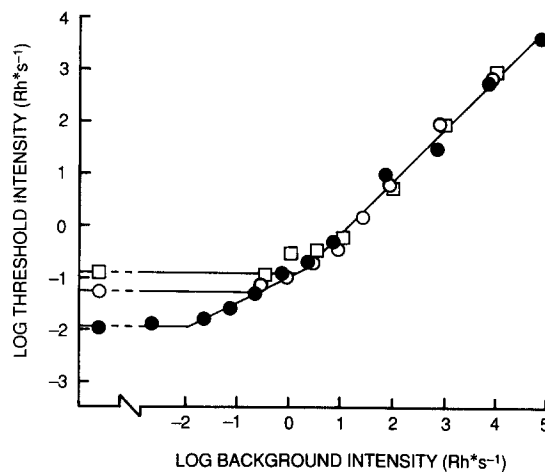
FIGURE 6. Increment thresholds of a ganglion cell ( filled circles ), a rod ( open circles ), and a horizontal cell ( squares ) as functions of log background intensity. For the two latter, "threshold" intensities were the intensities needed to produce a 2.8-mV criterion response. Step stimuli, full-field backgrounds. The abscissa (log background intensity) is common to all the cells. The ordinate, giving log threshold intensity, refers only to the ganglion cell. The rod data have been shifted down-
