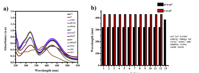
Fig. 5 (a) Selectivity studies and (b) wavelength changes of PTH-AB-PY towards various anions in UV-vis region.
