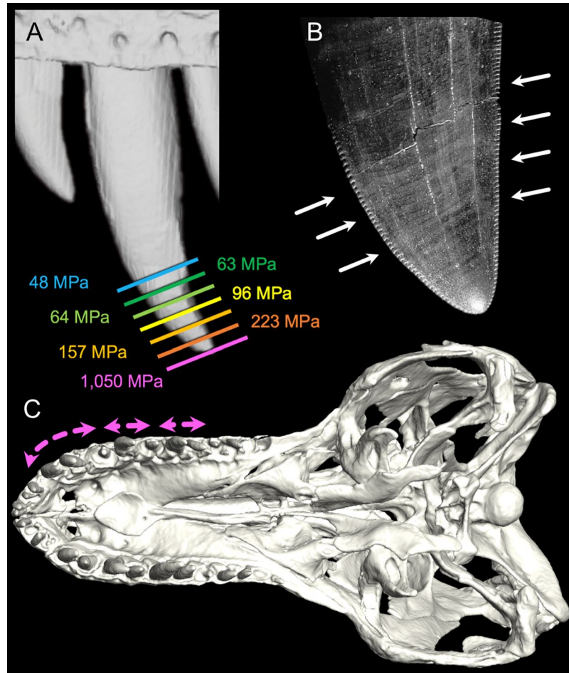
Figure 3. Tyrannosaurus rex dental functional morphology. (A) Exempler tooth pressures along the distal 37 mm of the left M5 of BHI 3033 (warmer colours indicate higher pressures), illustrating bone-penetrating shear stresses ( >65 MPa 4,39 ) for almost 25 mm of indentation depth. (B) Mesial and distal facing carinae (white arrows) helped direct pathways of bone fracture towards adjacent maxillary teeth (C) (ventral view of BHI 3033) that were also engaged during indentation, illustrating how the most procumbent maxillary tooth crowns collectively form a fracture arcade (pink arrows) due to pressures generated when biting. (Figure element in (A) derived from digital scan by Virtual Surfaces, Inc).
