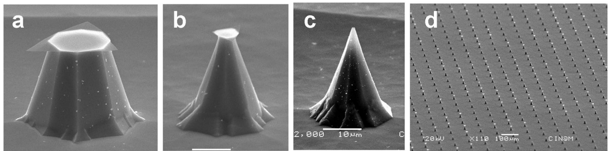
Figure 2. Silicon pyramids in a 75\ \mu\text{m} array etched in fresh 45 % KOH solution at T=63\ ^\circ\text{C} , sample holder rotation speed 170 r.p.m for 100 minutes (a), 110 minutes (b), 114 minutes, followed by an additional 4 minutes, after removal and inspection with a stereomicroscope (c). The 3 images are at the same magnification. (d) Large array of homogeneous pins at the end of the etching period. Of the 342 pins in this electron photomicrograph, 130 retain the "hat" that is subsequently removed in a pure water ultrasound bath. Manufacturing parameters: 75\ \mu\text{m} array; 750 ml fresh 45 % KOH; T=72\ ^\circ\text{C} ; 100 rpm. All the samples were tilted in the SEM at 70^\circ .
