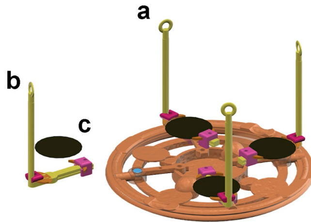
Figure 1. Drawing of a sample holder used for homogeneous KOH etching of multiple one-inch wafers (Autodesk 123 Design software). (a) Main support with magnets; (b) Arms for easy removal from etching solution; (c) One-inch (2.54 cm) diameter wafer to be etched.
