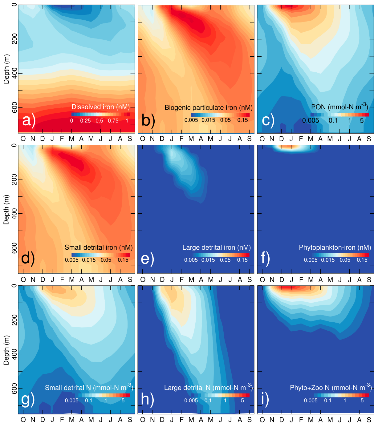
Figure 7. Seasonality of modeled distributions at the center of the polynya (Station 29; see Figure 1b for the location of the stations). (a) Dissolved iron (dFe), (b) biogenic particulate iron (bpFe), and (c) particulate organic nitrogen (PON). The second and third rows decompose bpFe and PON into their respective individual components (see section 2). The profiles are averaged over 2006–2013. Note the linear scale in (a) and the log scale in the other figures.
