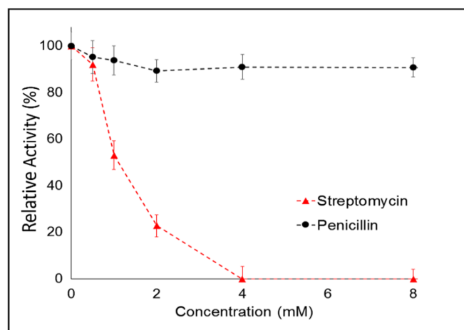
Figure 3 | Dose-response curve showing inhibition of RNase H activity by penicillin and streptomycin. The 100% of signal corresponds to the activity of 10 U/mL of RNase H (20 min at 25°C). Fluorescence values were collected after 40 min in the second step. Error bars represent the standard deviation (SD) calculated from triplicate experiments.
