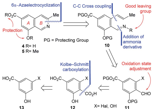
Scheme 1 Retrosynthetic analyses of ampullisine (4) and its derivative 5.
