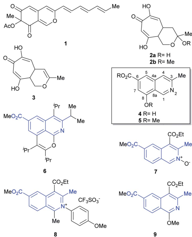
Fig. 1 Chemical structures of some polyketides (1–3) and ampullisine (4), isolated from Sepedonium species, as well as the semisynthetic ampullisine derivative (5) and structurally related, synthetic 3-methyl 6-carboxymethyl isoquinolines (6–9).
