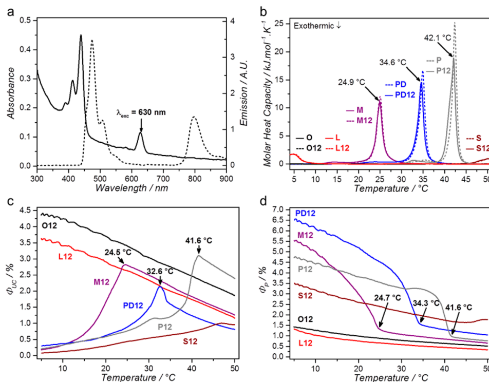
Figure 2. (Photo)physical characterization of upconverting liposomes. (a) Typical absorption (solid, left axis) and emission spectrum (dashed, right axis, \lambda_{exc} = 630 nm, intensity 80 \text{ mW cm}^{-2} ) of L12 liposomes ( [\text{DLPC}] = 1.0 \text{ mM} , [\mathbf{1}] = 0.5 \mu\text{M} , [\mathbf{2}] = 5 \mu\text{M} ) at 20^{\circ}\text{C} in 0.3 \text{ M} sodium sulfite PBS under air. (b) Differential scanning calorimetry thermograms between 5 and 50^{\circ}\text{C} of liposomes with TTA-UC dyes (O12, L12, M12, PD12, P12, and S12, solid) or without (O, L, M, PD, P, and S, dashed). The thermograms for liposomes S and S12 were recorded between 35 and 65^{\circ}\text{C} (Figure S3). Arrows indicate T_m of the dyed liposomes, where applicable. Measurements were performed in heating mode with a scanning rate of 1^{\circ}\text{C min}^{-1} at 3 \text{ atm} pressure. (c,d) Temperature evolution of the upconversion quantum yield ( \Phi_{UC} , c) and of the residual sensitizer phosphorescence quantum yield ( \Phi_p , d) of O12, L12, M12, PD12, P12, and S12. Samples were heated from 5 to 50^{\circ}\text{C} at a rate of 1^{\circ}\text{C min}^{-1} while continuously irradiated with 80 \text{ mW cm}^{-2} 630 \text{ nm} light, at 1.0 \text{ mM} lipid and [\mathbf{1}] = 0.5 \mu\text{M} and [\mathbf{2}] = 5 \mu\text{M} .
