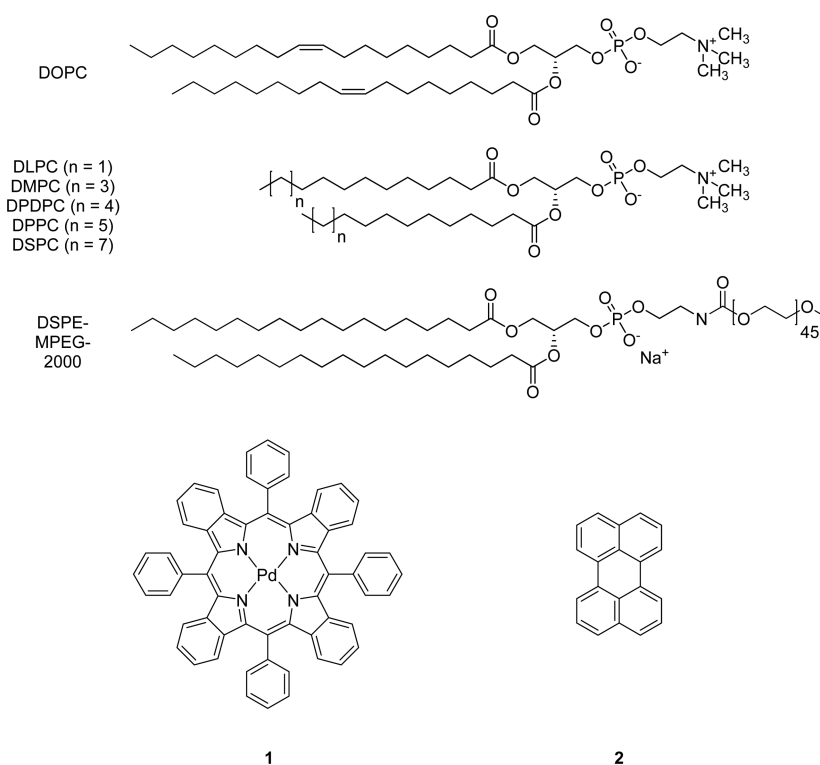
Figure 1. Chemical structures of DOPC, DLPC, DMPC, DPDPC, DPPC, DSPC, DSPE-mPEG-2000, palladium tetraphenyltetrabenzoporphyrin (1), and perylene (2).
