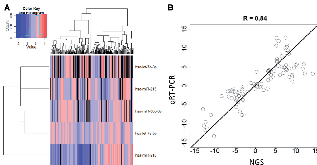
Figure 2. miRNA expression. (A) The heatmap visualization for the expression of the selected miRNAs across samples. (B) The comparison of NGS and RT-qPCR in quantification of mature miRNAs.
