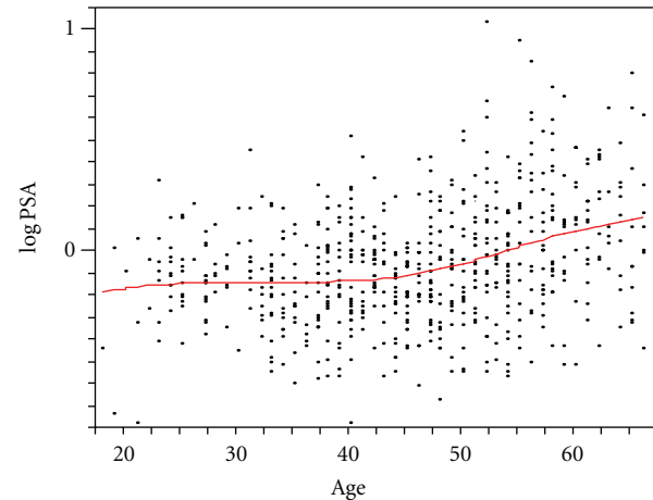
FIGURE 1: The graph shows the relationship between age and PSA (on a log scale) with a cubic spline with lambda set to 10,000.
