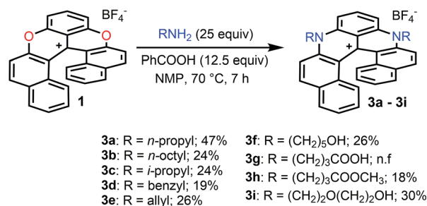
Fig. 3 Transformation of dioxo 1 into diaza 3a to 3i . n.f.: not formed.
