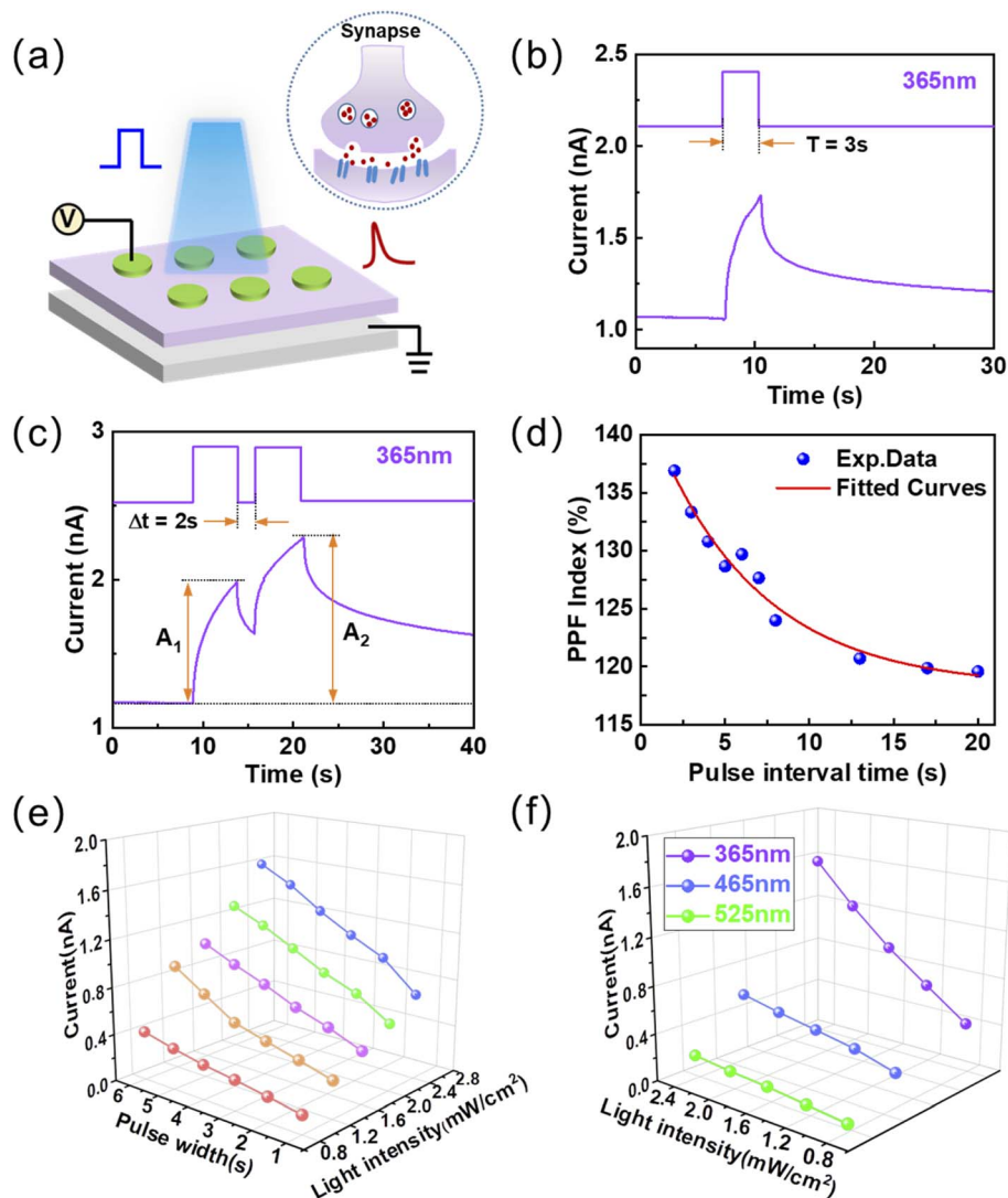
Fig. 2 The basic short-term visual memory properties. (a) Schematic diagram of the prepared ITO/TiO 2-x /p-Si devices and synapse structure. (b) EPSC triggered by a single light pulse of 365 nm with the intensity of 3.0 mW cm -2 . (c) EPSCs triggered by two continuous light pulses with an interval time of 2 s. (d) PPF index varies with pulse interval time. (e) Current as a function of light intensity and light pulse width. (f) Current variation with light intensity and wavelength.
