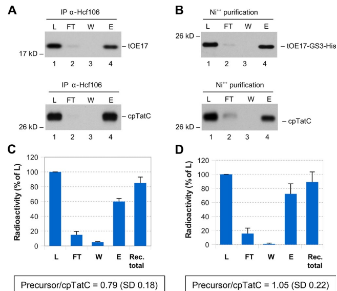
Figure 5. Affinity-purified precursor-bound receptor complex contains approximately one precursor protein per cpTatC. (A–D) Thylakoids were incubated with saturating amounts of tOE17 (A and C) or tOE17-GS3-His (B and D) in a binding reaction. Recovered thylakoids were solubilized with digitonin, and the insoluble pellet was removed by centrifugation. (A and C) The soluble extract (load; lane L) was incubated with \alpha -Hcf106 IgG beads, and the unbound material (lane FT) was removed after centrifugation. The recovered beads were washed (lane W) and then eluted with SDS buffer containing urea (lane E). (A) The tOE17 in the load and all fractions was detected by fluorography and cpTatC by immunoblotting. IP, immunoprecipitation. (C) The tOE17 in each fraction is shown as a percentage of starting material. Error bars represent the mean \pm SD ( n = 3 ). (B and D) The soluble digitonin extract from a binding reaction with tOE17-GS3-His (lane L) was incubated with Ni-nitrilotriacetic acid magnetic beads, and the unbound fraction (lane FT) was removed after magnetic separation. The beads were washed (lane W) and then eluted (lane E), and the fractions were subjected to fluorography and immunoblotting (B). The tOE17 in each fraction is displayed as the percentage of starting material. Error bars represent the mean \pm SD ( n = 3 ; D). The tOE17 and cpTatC were quantified in the elution (see Materials and methods). Total recovery (Rec. total) of tOE17 represents the amount of precursor present in the FT, W, and E fractions.
