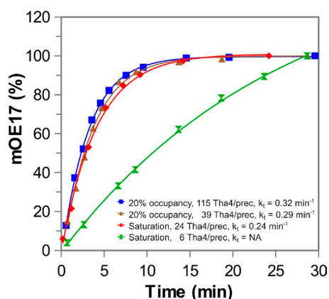
Figure 7. Analysis of the translocation phase in lag-subtracted chase reactions. The lag time from each chase experiment shown in Fig. 6 was subtracted from datasets, and the resulting data were plotted as the percentage of the final amount of mOE17 and fit to an exponential first-order equation (see Materials and methods). The k_t values for the translocation phase in experiments in which Tha4 per tOE17 was \geq 25 were 0.27 \text{ min}^{-1} (SD 0.04; n = 5 ) for tOE17-saturated receptors and 0.31 \text{ min}^{-1} (SD 0.05; n = 5 ) for low-occupancy receptor complexes. The plots of data shown are from a single representative experiment out of three independent repeats.
