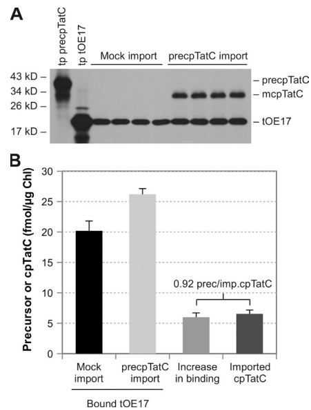
Figure 4. Import of cpTatC into chloroplasts increases thylakoid binding capacity by approximately one precursor per imported cpTatC. (A) Chloroplast import reactions were conducted with radiolabeled precpTatC or mock translation mixture (see Materials and methods). Recovered chloroplasts were treated with thermolysin, repurified, and used to isolate thylakoid membranes. Parallel binding assays were conducted with saturating concentrations of tOE17 (see Materials and methods). A fluorogram of samples recovered from binding assays is shown. tp, translation product. (B) Radiolabeled imported cpTatC and tOE17 were quantified by scintillation counting. The increase in binding was obtained as the difference in the amount of bound tOE17 between thylakoids with imported (imp.) cpTatC and thylakoids from the mock import reaction. Error bars represent the mean \pm SD ( n = 3 ). Chl, chlorophyll.
