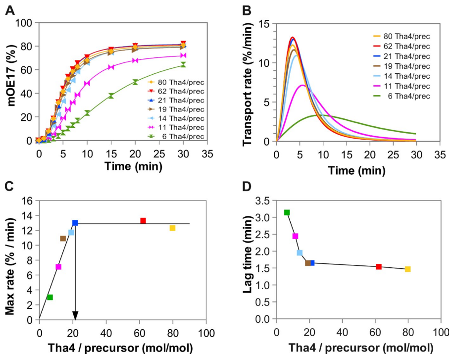
Figure 8. The Tha4 oligomer required to transport an OE17 precursor contains ~26 Tha4 protomers. Chase reactions with tOE17-saturated membranes were conducted with different amounts of IVT Tha4 (see Materials and methods). (A) Transport of tOE17 was quantified as the amount of mOE17 produced and plotted as the percentage of tOE17 at time 0, and the data were fit to a sigmoidal equation (see Materials and methods). (B) Instantaneous transport rates for each chase reaction were estimated with the first derivative of the fitted curves. (C) The amount of Tha4 (quantitative immunoblotting) per precursor protein (radio-label) was estimated for each chase reaction (see Materials and methods) and plotted versus the highest instantaneous transport rates (Max rate). Regression lines for the chase reactions with <25 Tha4/tOE17 and for the chase reactions with 21–80 Tha4/tOE17 are shown. The intercept of the two lines (arrow) represents the Tha4 sufficiency point (21 Tha4 per precursor) for transport of tOE17. The mean sufficiency point for the three independent measurements was 26 (SD 6.3). (D) Lag times were estimated, as in Fig. 6, and plotted versus Tha4/tOE17. Data points in C and D are colored and correspond to the chase reactions shown in A and B. The plots of data in the figure are from a single representative experiment out of three independent repeats.
