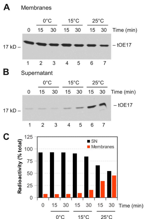
Figure 1. The tOE17 precursor binds to the receptor complex with high affinity and a low rate of dissociation. (A and B) Thylakoid membranes were incubated with saturating amounts of radiolabeled tOE17, as determined in Fig. 3. Membranes were then recovered, washed twice, and incubated with saturating amounts of unlabeled tOE17 at 0, 15, or 25°C. At time points, aliquots were removed, and the membrane (A) and supernatant (B) fractions were analyzed by SDS-PAGE and fluorography. (C) Radioactivity was measured by scintillation counting of extracted gel slices and plotted as a percentage of the total for each time point. The data are from a single experiment, which is representative of several similar experiments conducted at the temperatures shown. SN, supernatant.
