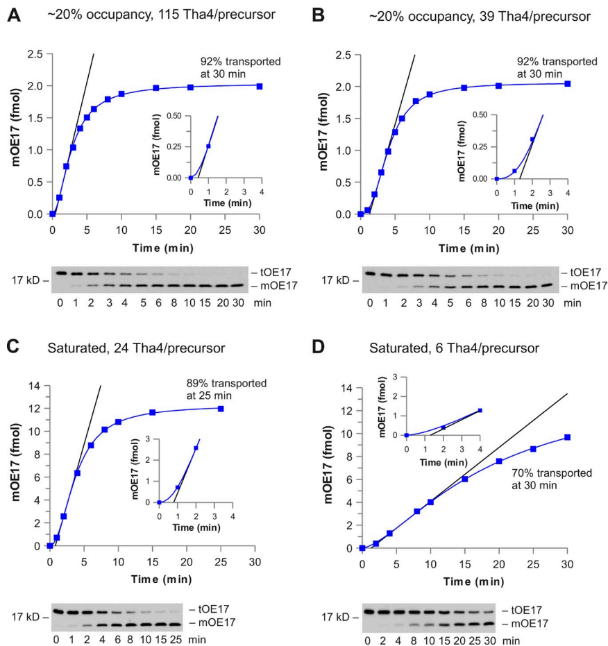
Figure 6. Kinetics of bound tOE17 transport in 20% precursor-saturated and 100% saturated membranes with sufficient and insufficient Tha4. (A–D) Thylakoid membranes were incubated in binding reactions with concentrations of tOE17 that resulted in 20% (A and B) or 100% (C and D) saturation of receptor complexes. After binding, thylakoids were incubated with IVT Tha4 (A and C) or with mock translation mixture (B and D). Transport of bound tOE17 (chase) was started with ATP and transfer to a 15°C light bath followed by sampling at time points (see Materials and methods). The transported OE17 (mOE17) was fit to a sigmoidal equation (blue lines). Tangent lines (black) were drawn at the inflection point of each curve and used to determine the lag times (see Materials and methods). Fluorograms of chase reactions are displayed below the panels. In the plots, note the differences in y-axis scales between 20% saturated and 100% saturated membranes. The data are from a single representative experiment out of three independent repeats.
