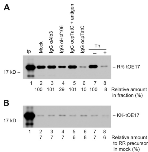
Figure 2. The tOE17 precursor binds directly and specifically to cpTatC. (A and B) Thylakoid membranes were treated with 0.5 mg/ml IgGs (lanes 3–6) in the absence or presence of ~4 μM antigen (lane 5) for 1 h on ice and then incubated with saturating amounts (determined in Fig. 3) of radiolabeled RR-tOE17 (A, translation product [tp] lane 1) or nonfunctional KK-tOE17 (B, tp lane 1). Alternatively, thylakoids were treated or mock treated with 100 μg/ml thermolysin (Th; lanes 7 and 8) for 40 min on ice. Proteolysis was terminated with EDTA, after which membranes were recovered, washed with IB 5 mM EDTA, resuspended in IBM, and then incubated with saturating amounts of RR-tOE17 (A) or KK-tOE17 (B) for 60 min. Membranes were recovered, washed, and analyzed (see Materials and methods).
