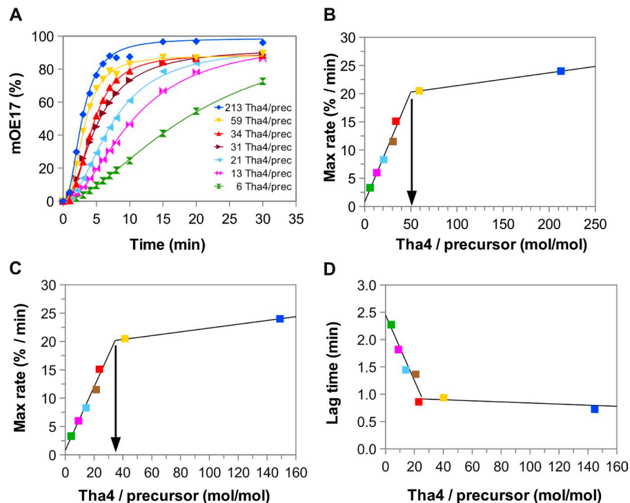
Figure 9. Estimation of the minimal Tha4 oligomer size for optimal transport relying only on endogenous Tha4. Binding reactions were conducted with varying concentrations of tOE17. Chase reactions were conducted without added Tha4 (see Materials and methods). (A) The amount of transported OE17 (mOE17) was plotted as the percentage of the total amount of tOE17 at time 0 and fit to a sigmoidal equation. (B) Tha4 per tOE17 for each chase reaction (see Materials and methods) was plotted versus the highest instantaneous transport rates (Max rate), as estimated from the first derivative of the fitted sigmoidal curves. (C) Tha4 concentrations were corrected by an estimate of nonavailable Tha4 and plotted versus the highest instantaneous transport rates. A regression line was drawn for chase reactions with increasing highest instantaneous rates, and a straight line was drawn for the two chase reactions that had achieved the maximum rate. (B and C) The intercept between the two lines indicates the Tha4 sufficiency point (arrows). (D) The lag time for each chase reaction was plotted versus the corrected Tha4/tOE17 ratio. The data points in B, C, and D are colored and correspond to the chase reactions shown in A. The data are from a single representative experiment out of two independent repeats. The corrected Tha4/tOE17 sufficiency point for the two experiments was 31.
