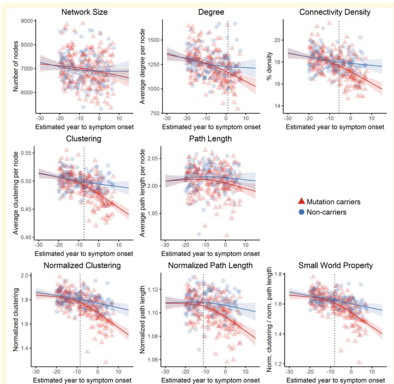
Figure 3 Grey matter network properties by estimated year of onset at baseline between mutation carriers and non-carriers.
