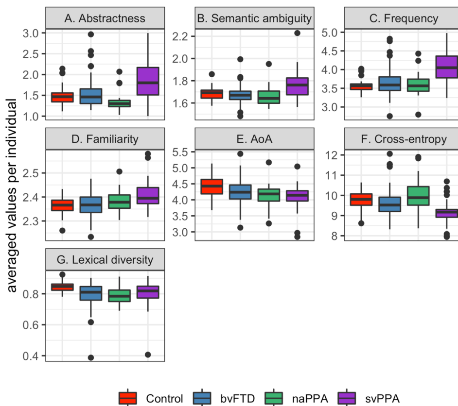
Figure 2: Median, 1SD, 25th-75th percentile and outliers of abstractness scores, semantic ambiguity ratings, word frequency, word familiarity, and age of acquisition of nouns; and cross-entropy estimation and lexical diversity across all words.
