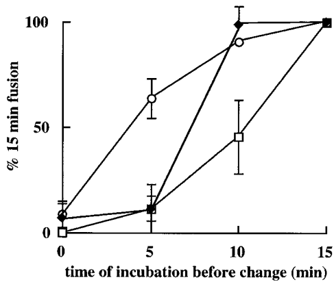
Figure 3. Luminal \text{Ca}^{2+} is required in a late phase of late endosome-lysosome fusion. BAPTA (5 mM; \blacklozenge ) and GDI (20 \mu\text{M} ; \circ ) were added to the ongoing content mixing assay at different times after the start and the effect of these inhibitors on the rest of the incubation period was monitored. First, as controls, a content mixing assay was carried out under standard conditions except that the incubation time at 37^\circ\text{C} was 15 min, resulting in the 100% value by definition. Second, content mixing assays were carried out under standard conditions except that after defined times at 37^\circ\text{C} , the assays were stopped by placing the incubation tubes in ice ( \square ). Data are presented as mean \pm SEM of three experiments.
