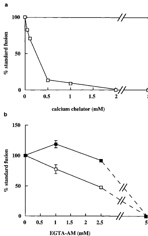
Figure 2. Inhibition of late endosome–lysosome content mixing by EGTA-AM. (a) Dose–response curve of inhibition with EGTA-AM (□) or EGTA (●) present at the concentrations stated throughout a standard incubation. For treatment with EGTA-AM, results are expressed as the percentage of the total immunoprecipitable counts that had formed within the late endosome–lysosome hybrid organelles in the presence of DMSO. (b) Effects of organelle pretreatment with EGTA-AM on content mixing in a standard incubation. (□) Late endosomes; and (■) lysosomes. Data are presented as mean \pm SEM of three experiments. The solid line depicts the range of EGTA-AM concentration where inhibition can be reversed by the addition of \text{CaCl}_2 . At 5 mM EGTA-AM, addition of \text{CaCl}_2 does not reverse inhibition.
