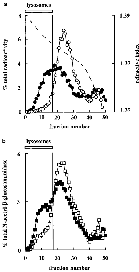
Figure 4. The reformation of lysosomes from hybrid organelles. A hybrid organelle-enriched fraction from rat liver containing endocytosed ^{125}\text{I} -labeled bpIgA was resuspended in STKM and incubated for 10 min at 37^\circ\text{C} (closed symbols), or kept on ice (open symbols) in the presence of an ATP-regenerating system and 1 mM ATP. The incubation mixture (0.7 ml) was loaded onto a 4.2-ml 12–30% Nycodenz gradient prepared on top of a cushion of 0.3 ml 45% Nycodenz. After centrifugation, followed by fractionation, the distributions of radioactivity (a) and N -acetyl- \beta -glucosaminidase (b) were measured. A representative experiment is shown. The lysosomal region of the gradient is indicated by the bars to the left of the vertical lines. The broken line in (a) shows the refractive index of gradient fractions after centrifugation.
