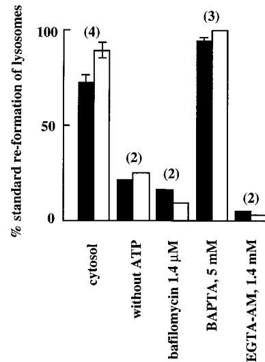
Figure 7. Requirements for the reformation of lysosomes from hybrid organelles. Lysosome reformation was calculated from the recovery of ^{125}\text{I} -labeled bpIgA (solid bars) and N -acetyl- \beta -glucosaminidase (open bars) at the lysosomal position on a 12–30% Nycodenz gradient, after incubation as indicated. Results are expressed as percentages of lysosome reformation obtained on the same day under standard conditions, i.e., with a hybrid organelle enriched fraction isolated from rat liver incubated in STKM for 10 min at 37^\circ\text{C} in the presence of an ATP-regenerating system and 1 mM ATP. Cytosol, bafilomycin A1 (1.4 \mu\text{M} ), BAPTA (5 mM), and EGTA-AM (1.4 mM) when added, were present throughout a standard reformation assay. In the cases of treatment with bafilomycin A1 and EGTA-AM, the results are expressed as the percentage of lysosome reformation obtained on the same day under standard conditions in the presence of DMSO. The numbers above the bars indicate the number of experiments. Data are presented as mean \pm SEM (range errors on pairs too small to show).
