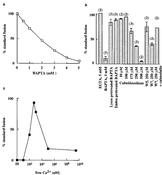
Figure 1. Inhibition of late endosome–lysosome content mixing by BAPTA. (a) Dose–response curve of inhibition. BAPTA at the concentrations stated was present throughout a standard incubation (i.e., for 10 min at 37^\circ\text{C} in the presence of cytosol), an ATP-regenerating system, 1 mM ATP, and 1 mM GTP. The results are expressed as the percentage of the total immunoprecipitable counts that had formed within late endosome–lysosome hybrid organelles. Data are from a representative experiment. (b) Effects on content mixing of EGTA, pretreatment of organelles with BAPTA, or calmodulin antagonists. Content mixing was not inhibited by 5 mM EGTA in contrast to the effect of 5 mM BAPTA. Pretreatment of lysosomes (lysos) or late endosomes (endos) with 5 mM BAPTA was for 15 min on ice. The calmodulin antagonists (calmidazolium at concentrations stated or W5 and W7 each at 250 \mu\text{M} ) without or with calmodulin (60 U) were present throughout standard incubations. For the calmodulin antagonists, the results are expressed as the percentage of the total immunoprecipitable counts that were formed within late endosome–lysosome hybrid organelles in the presence of DMSO. The numbers above the bars indicate the number of experiments. Data are presented as mean \pm SEM or range. (c) Reversal of BAPTA inhibition of content mixing by addition of \text{CaCl}_2 . The standard content mixing assay was carried out in the presence of 5 mM BAPTA together with different concentrations of \text{CaCl}_2 , resulting in the calculated free \text{Ca}^{2+} concentrations shown (for method of calculation see Materials and Methods).
