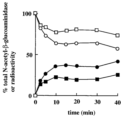
Figure 6. Time course of the reformation of lysosomes from hybrid organelles. A hybrid organelle-enriched fraction, from the rat liver containing endocytosed ^{125}\text{I} -labeled bpIgA, was incubated in STKM for different times at 37^\circ\text{C} in the presence of an ATP-regenerating system and 1 mM ATP. The incubation mixtures were loaded onto 12–30% Nycodenz gradients and, after centrifugation and fractionation, the amounts of radioactivity (● and ○) and N -acetyl- \beta -glucosaminidase (■ and □) in the fractions containing hybrids (open symbols) and lysosomes (solid symbols) were measured. The results are expressed after subtracting the amounts of radioactivity (7% of total on gradient) and N -acetyl- \beta -glucosaminidase (16% of total on gradient) found at the lysosomal position after centrifugation of hybrid organelles kept on ice.
