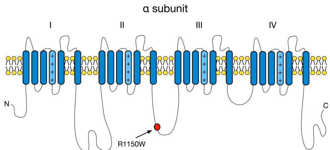
FIGURE 1: Nav1.7 alpha-subunit structure showing the location of amino acid affected by investigated common polymorphism rs6746030 is marked with the arrow
