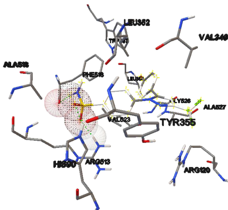
Fig. 1 Hydrogen bond interaction between the sulfonamide group of SC58 and three amino acid residues, HIS90, ARG513 and PHE518, of Cyclooxygenase-2 (1CX2)
