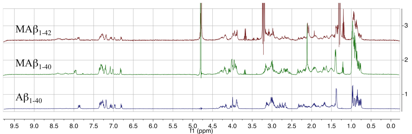
Fig 5. ^1\text{H} NMR of \text{MA}\beta_{1-40} and \text{MA}\beta_{1-42} compared with \text{A}\beta_{1-40} . Samples of \text{MA}\beta in water are diluted to 100 \mu\text{M} in 100 mM phosphate buffer pH 7 in \text{D}_2\text{O} . Synthetic \text{A}\beta_{1-40} is dissolved in NaOD and diluted to 100 \mu\text{M} under the same conditions. Signals at 4.75 ppm correspond to \text{H}_2\text{O} , and signals at 3.25 ppm and 1.25 ppm correspond to traces of ethanol.
