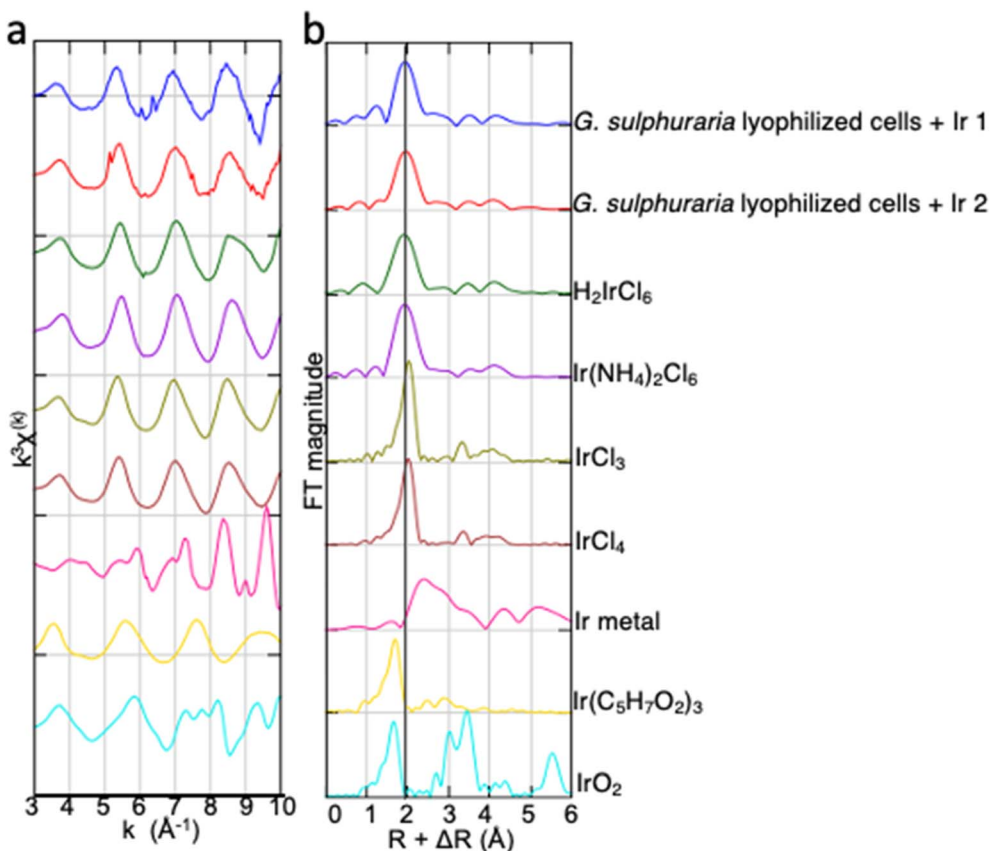
Fig. 7 EXAFS spectra of the Ir adsorbed on lyophilized G. sulphuraria cells and reference materials. (a) k^3 -weighted \chi(k) EXAFS oscillations and (b) the corresponding RFS.
