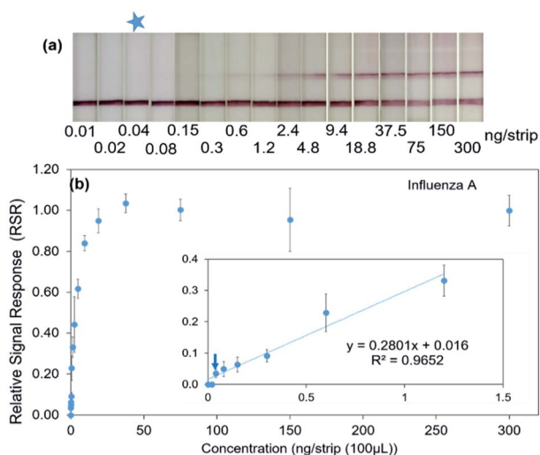
Fig. 3 (a) Result visualization and (b) the relative signal response against the presence of influenza A proteins, ranged from 0–300 ng per test. The increase in the signal was shown to be correlated to the increase of influenza A protein. Error bars were obtained from 3 separate experiments. Arrow and star indicate LOD.
