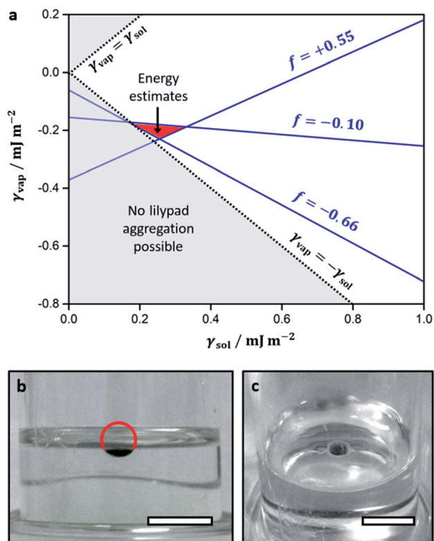
Fig. 4 The surface energies of a lily pad aggregate may be estimated by plotting the possible surface energies for three aggregate geometries (shown in blue) and identifying the area of intersection (red) (a). Side (b) and top-down (c) views are shown for a typical lily pad aggregate, where f = -0.66 , R = 1.34 mm and V = 0.77 mm 3 . Scale bars represent 5 mm in both images. The aggregate occupies a fraction of a sphere, the full circumference of which is delineated in red.
