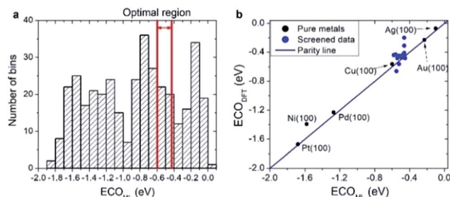
Fig. 6 (a) A histogram of the predicted *CO binding energy ( E_{\text{CO,ML}} ) using the active KRR machine using W_d^{\text{MTO}} and \chi_p as descriptors after screening 372 transition metal-based alloys. (b) The *CO binding energy comparison between the DFT calculation ( E_{\text{CO,DFT}} ) and the prediction by machine learning ( E_{\text{CO,ML}} ) for 15 candidates selected from (a).
