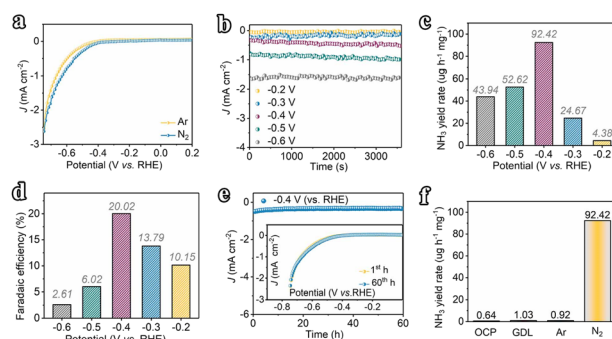
Fig. 3 (a) LSV curves of the Fe nanochain electrode recorded for \text{N}_2 electro-fixation in \text{N}_2 -saturated and Ar-saturated 0.1 M \text{Na}_2\text{SO}_4 solution (scan rate 5 \text{ mV s}^{-1} ). (b) Chronoamperometry curves of the Fe nanochain at -0.2 – 0.6 \text{ V} (vs. RHE). (c and d) \text{NH}_3 yields and faradaic efficiencies of the Fe nanochain at -0.2 – 0.6 \text{ V} (vs. RHE). (e) Stability test for 60 h at -0.4 \text{ V} (vs. RHE); the inset of (e) shows LSVs of the electrode before and after the stability test. (f) \text{NH}_3 yields of the Fe nanochain at -0.4 \text{ V} (vs. RHE) under different testing conditions.
